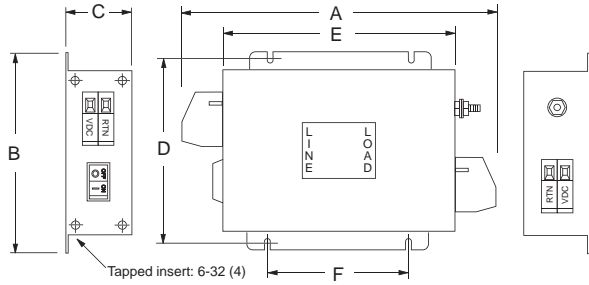
Typical Dimensions: Mounting Slots (4): .260 x .39 [6.6 x 9.9]
